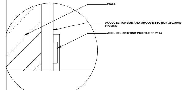
WALL CORNER PANELING DETAIL
