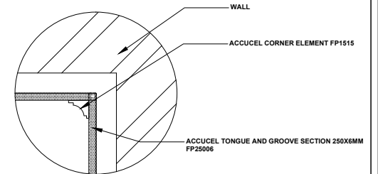
WALL CORNER PANELING DETAIL
