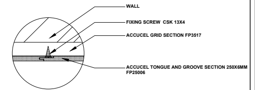
PANELING DETAIL
